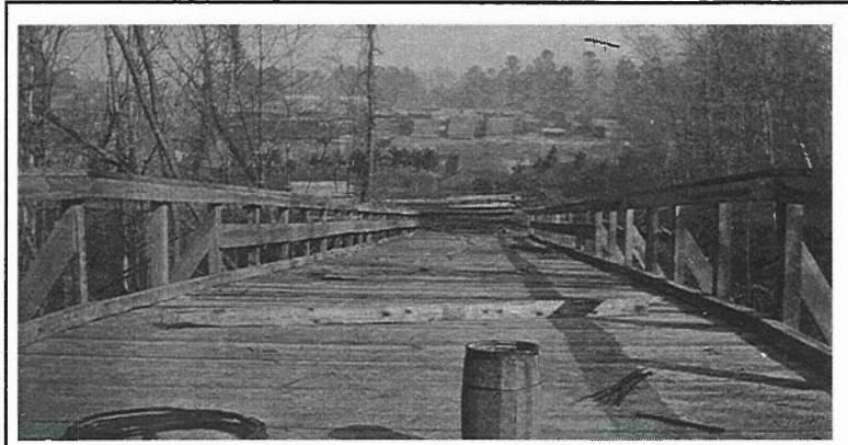
Figure 23. Temporary bridge under construction. To the north is the lumber storage yard and rail spur (courtesy of SCE&G).
