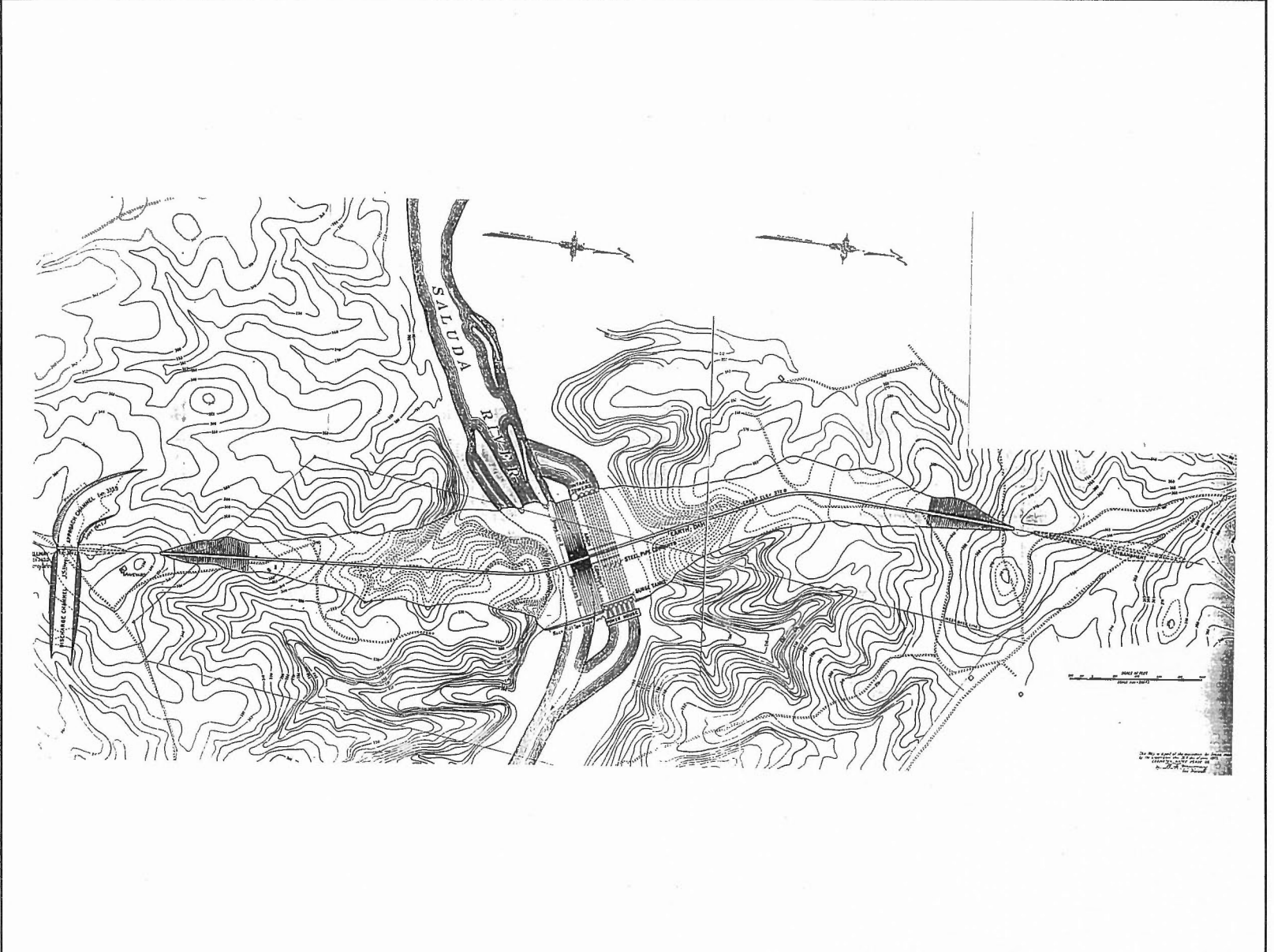
Figure 21. Pre-construction map of the dam area (Federal Power Regulatory Commission, Permit 516, Exhibit K, Items 516-11 and 12).
