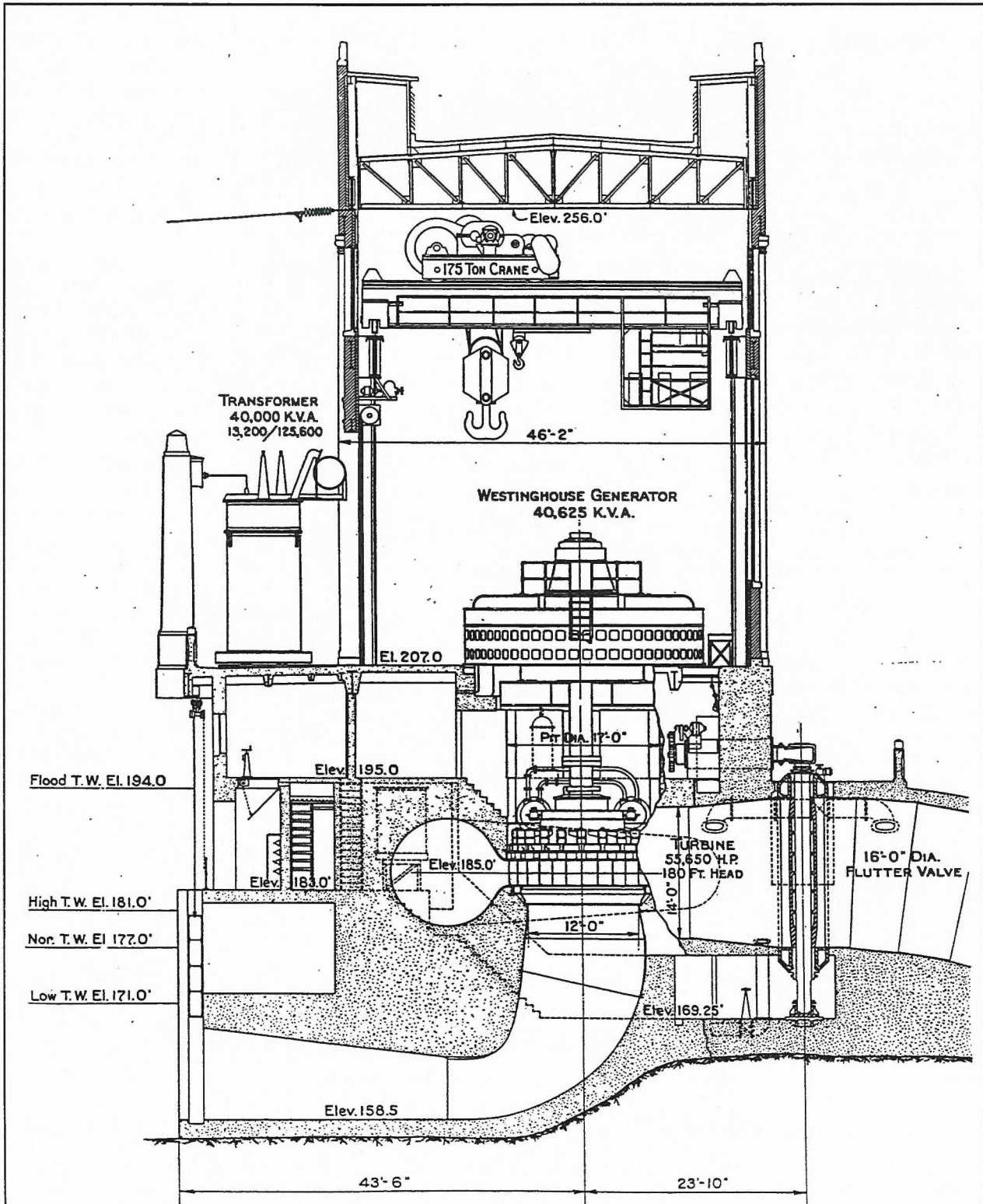
Figure 31. Cross section view of the Saluda powerhouse (adapted from Associated Gas & Electric System n.d.:29).
