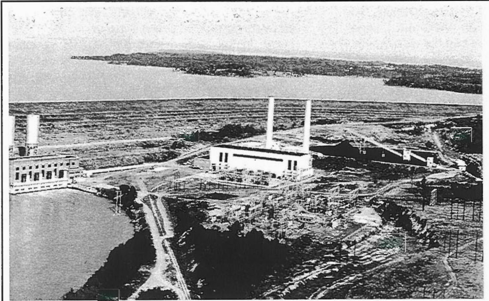
Figure 35. View of the completed McMeekin Station, May 8, 1961. Note how the ridge to the east continues to be cut away (courtesy of SCE&G).
