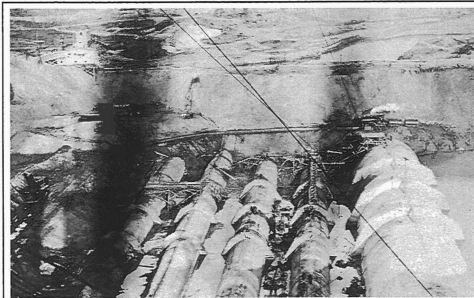
Figure 25. View of the penstock construction on January 3, 1929 looking east, into the survey area. Note the extensive clearing and ground disturbance from construction. (Duncan, Kinard, Sanders, and Tucker Family Album, 1928-1929; Courtesy of South Caroliniana Library, University of South Carolina).
