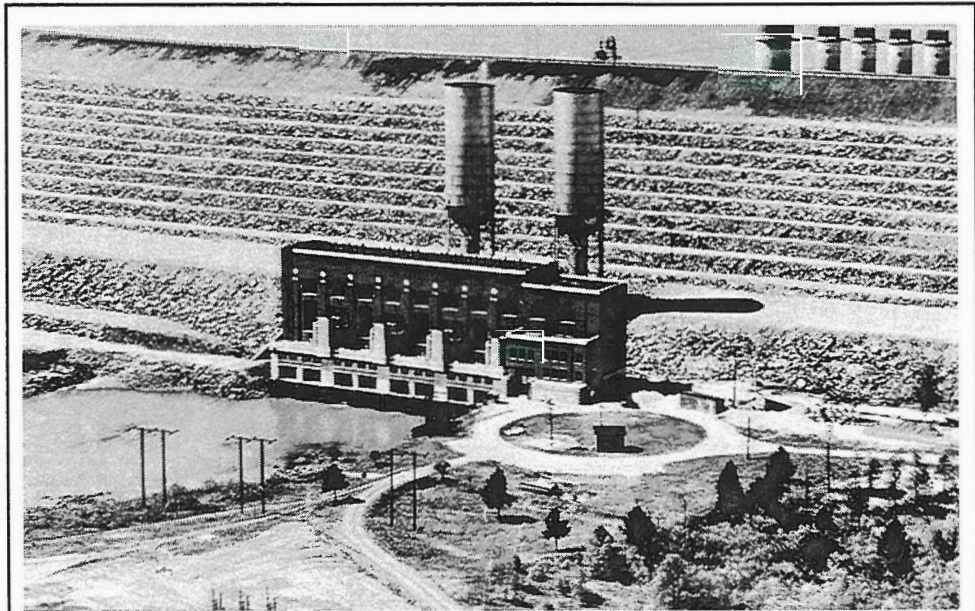
Figure 30. Airplane view of the Saluda dam and powerhouse from about 1944. The arched conduit is barely visible, having been extended when rip rap was added (courtesy of SCE&G).
