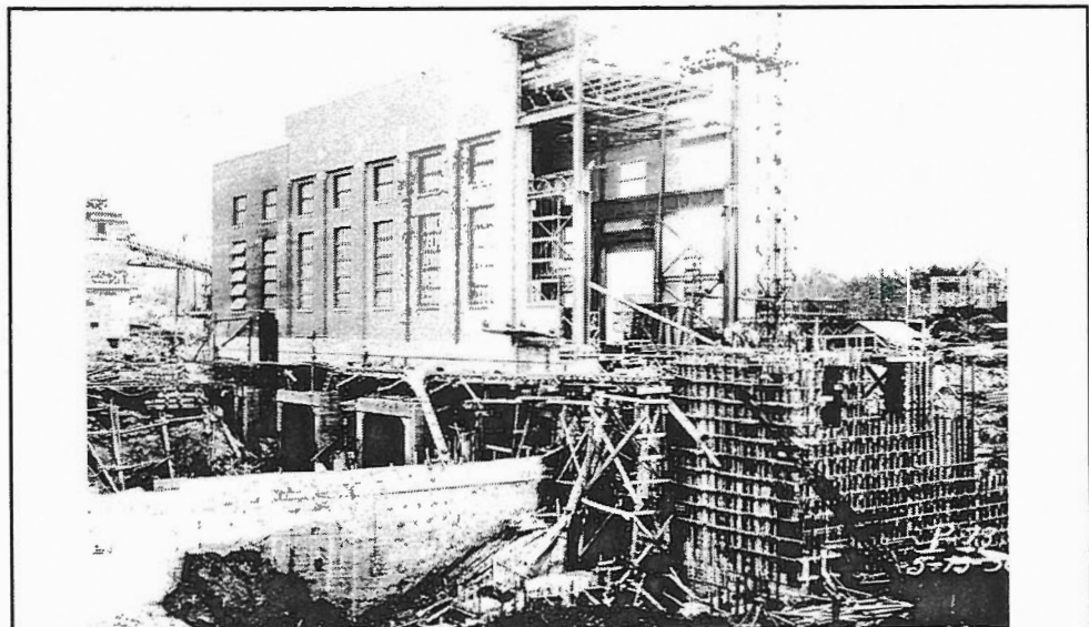
Figure 28. View of the Saluda Hydroelectric powerhouse under construction, looking northeast. At the right hand side is the substation lot (courtesy of SCE&G).
