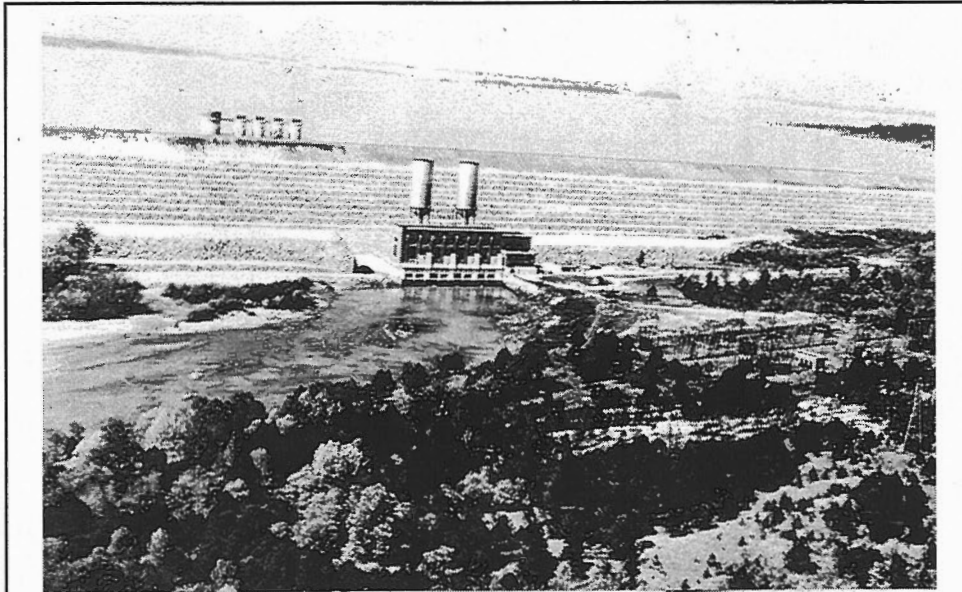
Figure 29. View of the completed Saluda Hydroelectric project, ca. 1945. The construction area is being re-vegetated. The arched conduit is still clearly visible to the left of the powerhouse. Also visible on the right side of the photograph is the brick substation (courtesy of SCE&G).
